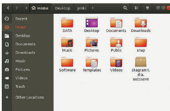
Figure 3.18: File Explorer
